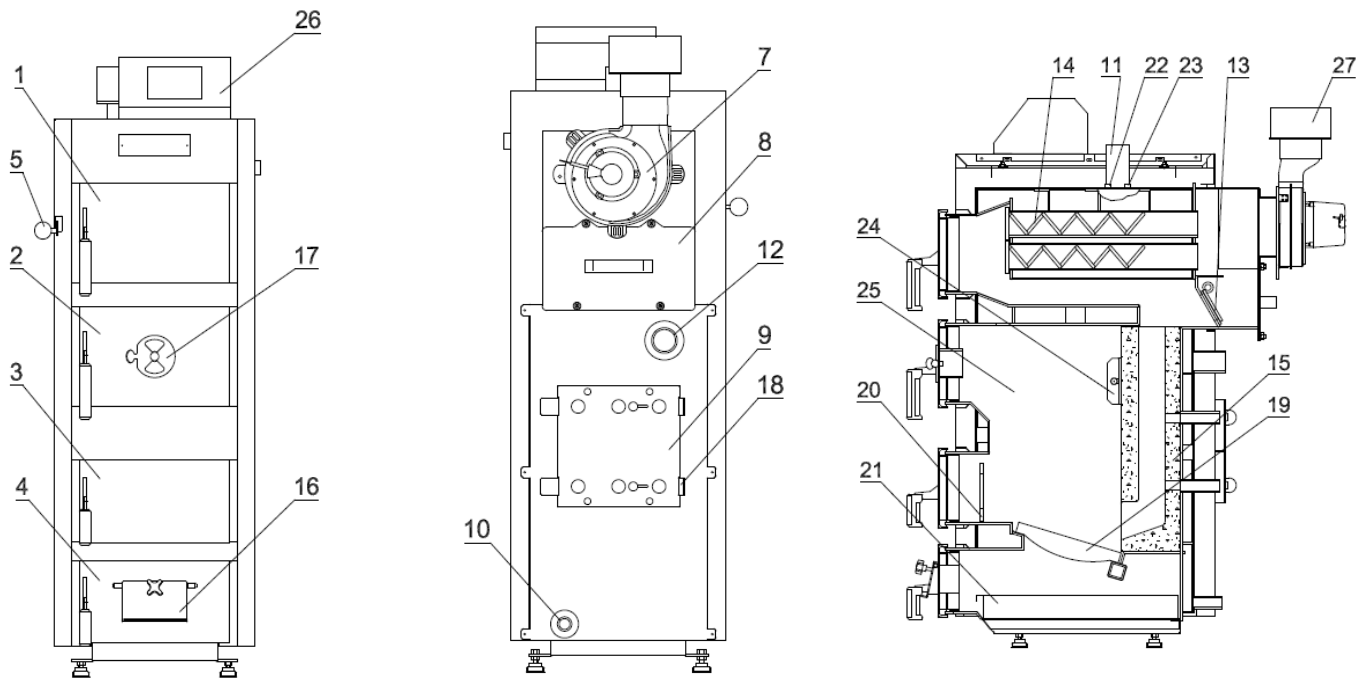
CROSS-SECTION OF THE SEM DUOPELL BOILER 16
